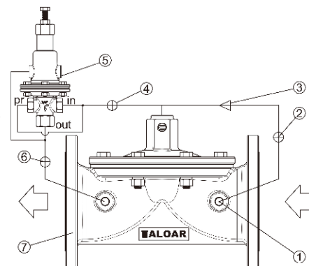
Piping Diagram
