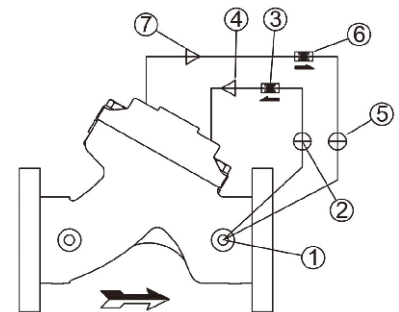
Piping Diagram
