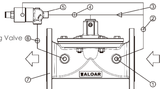
Piping Diagram
